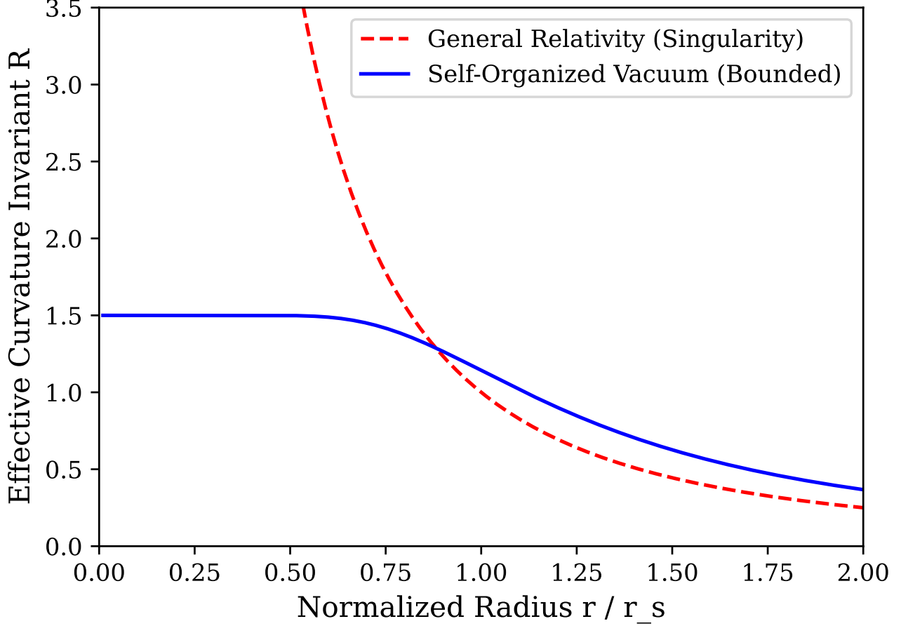
FIG. 3. Phenomenological core regularization (Test 4): effective Kretschmann proxy near r \rightarrow 0 . Classical Schwarzschild curvature diverges (dashed). The saturating pressure Eq. (42) yields a bounded proxy (solid). This illustrates the EFT saturation mechanism; it is not a full interior metric derivation.
