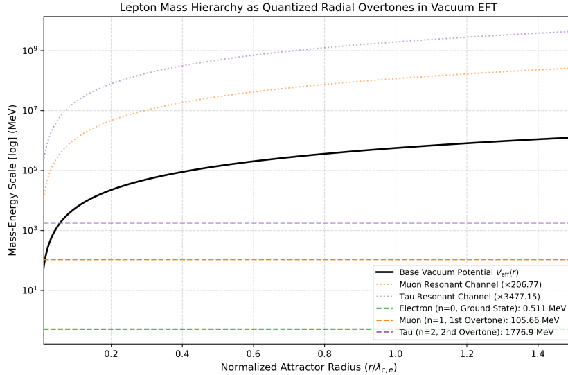
Figure 1: The mass hierarchy of charged leptons ( e, \mu, \tau ) formulated as quantized radial overtones within the effective vacuum response potential V_{\text{eff}}(r) .
