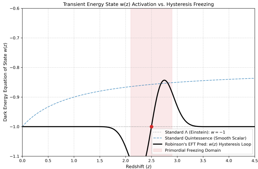
Figure 2: The transient activation profile of the dark energy equation of state w(z) driven by the non-equilibrium hysteresis freezing mechanism near z_{\text{crit}} = 2.5 , contrasted against standard quintessence alternatives.
