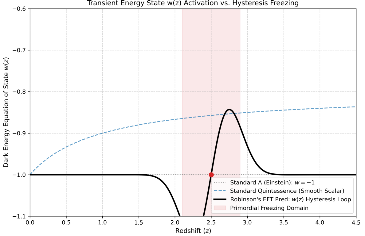
Figure 2: The transient activation profile of the dark energy equation of state w(z) driven by the non-equilibrium hysteresis freezing mechanism near z_{\text{crit}} = 2.5 , contrasted against standard quintessence alternatives.
