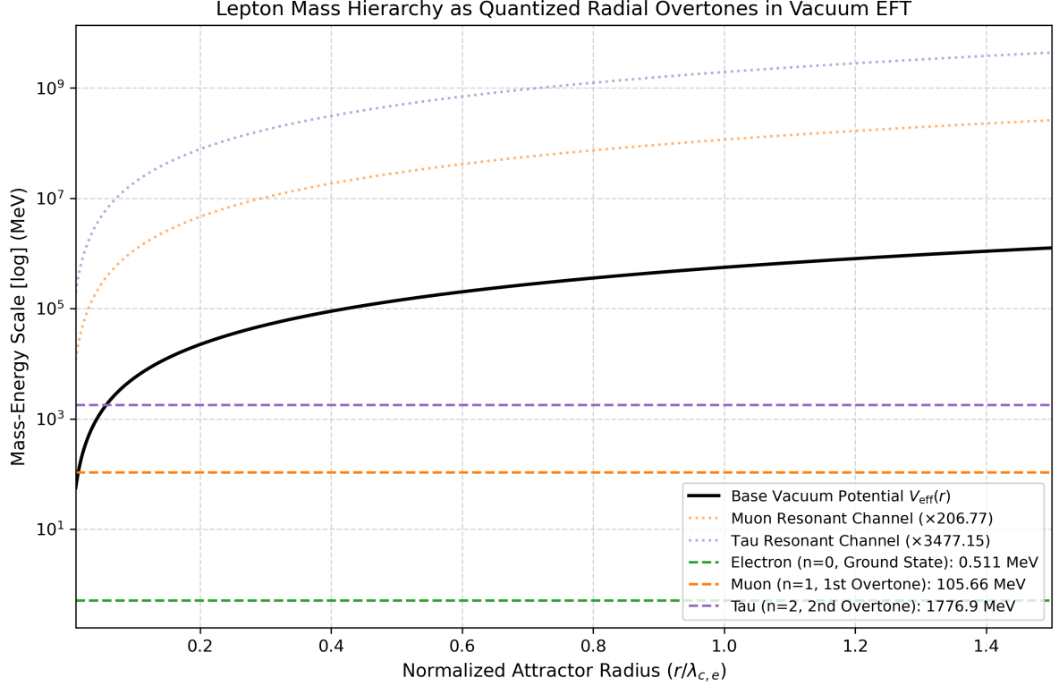
Figure 1: The mass hierarchy of charged leptons ( e, \mu, \tau ) formulated as quantized radial overtones within the effective vacuum response potential V_{\text{eff}}(r) .
