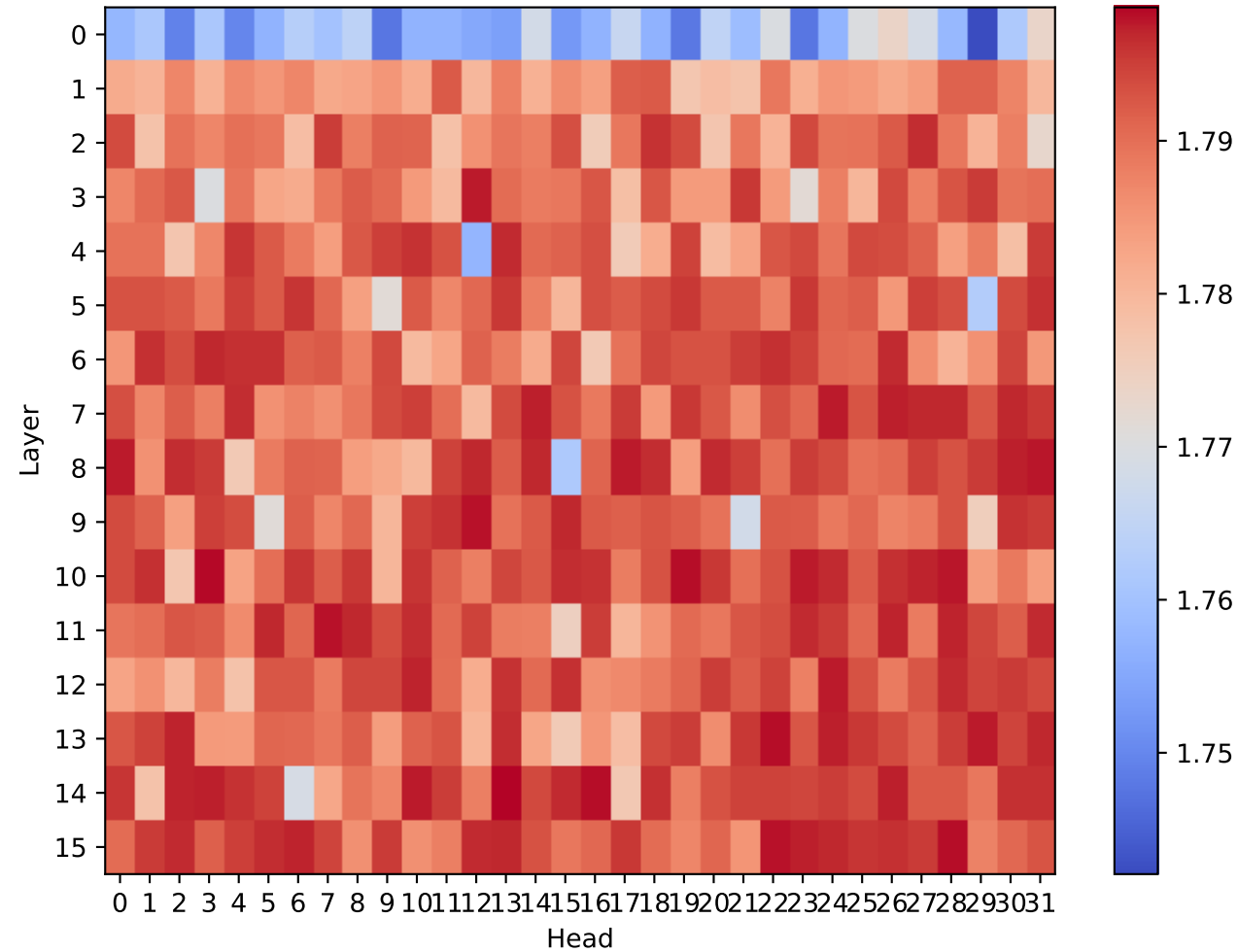
Attention Entropy
