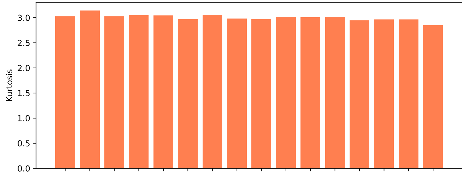
Hidden State Kurtosis per Layer (higher = more outlier)
