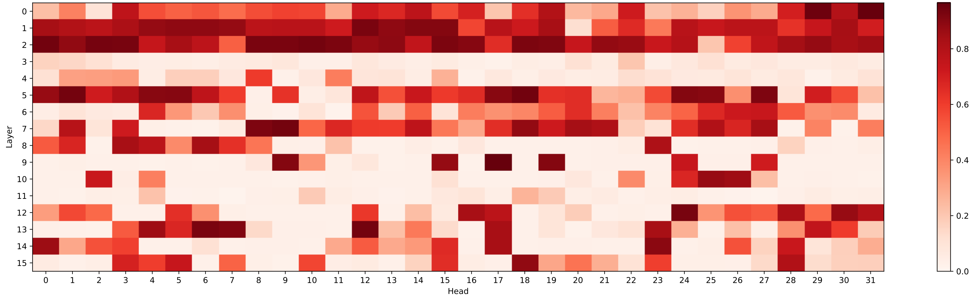
Attention Sink: Mean Prob on Token 0
