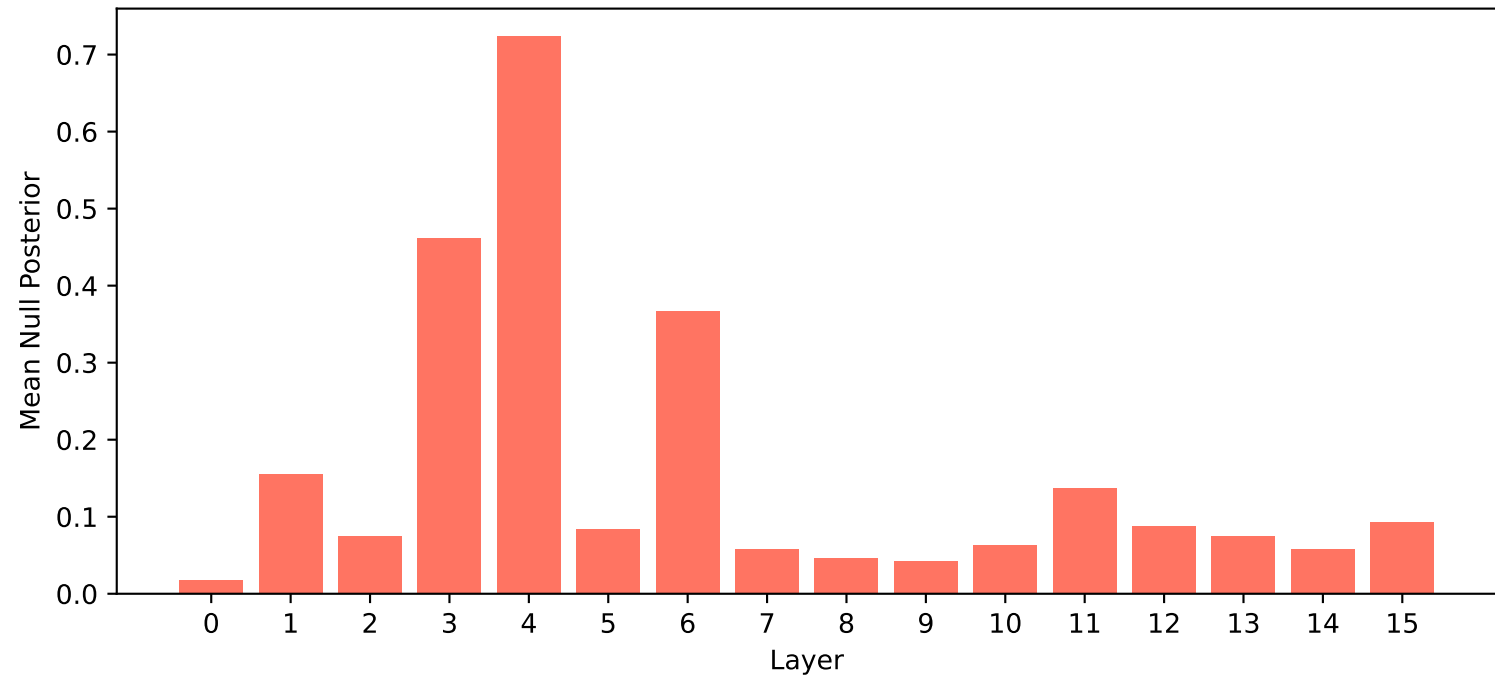
OASIS: Null Posterior per Layer (mass routed to null space)
