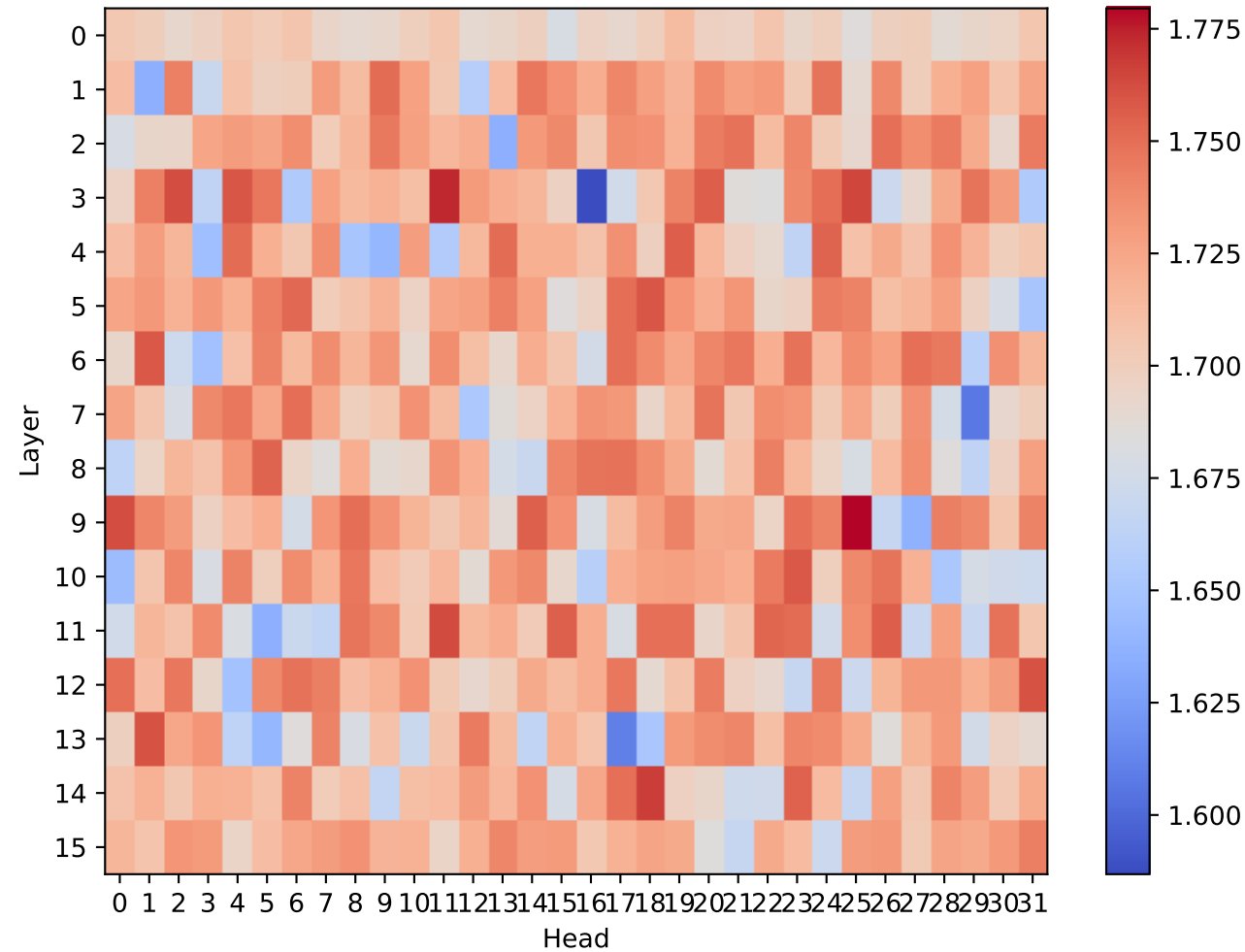
Attention Entropy
