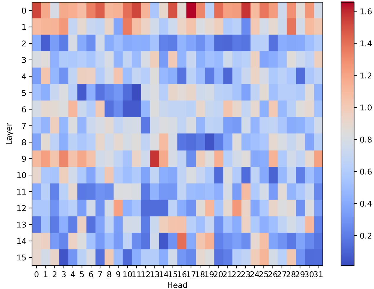
Attention Entropy
