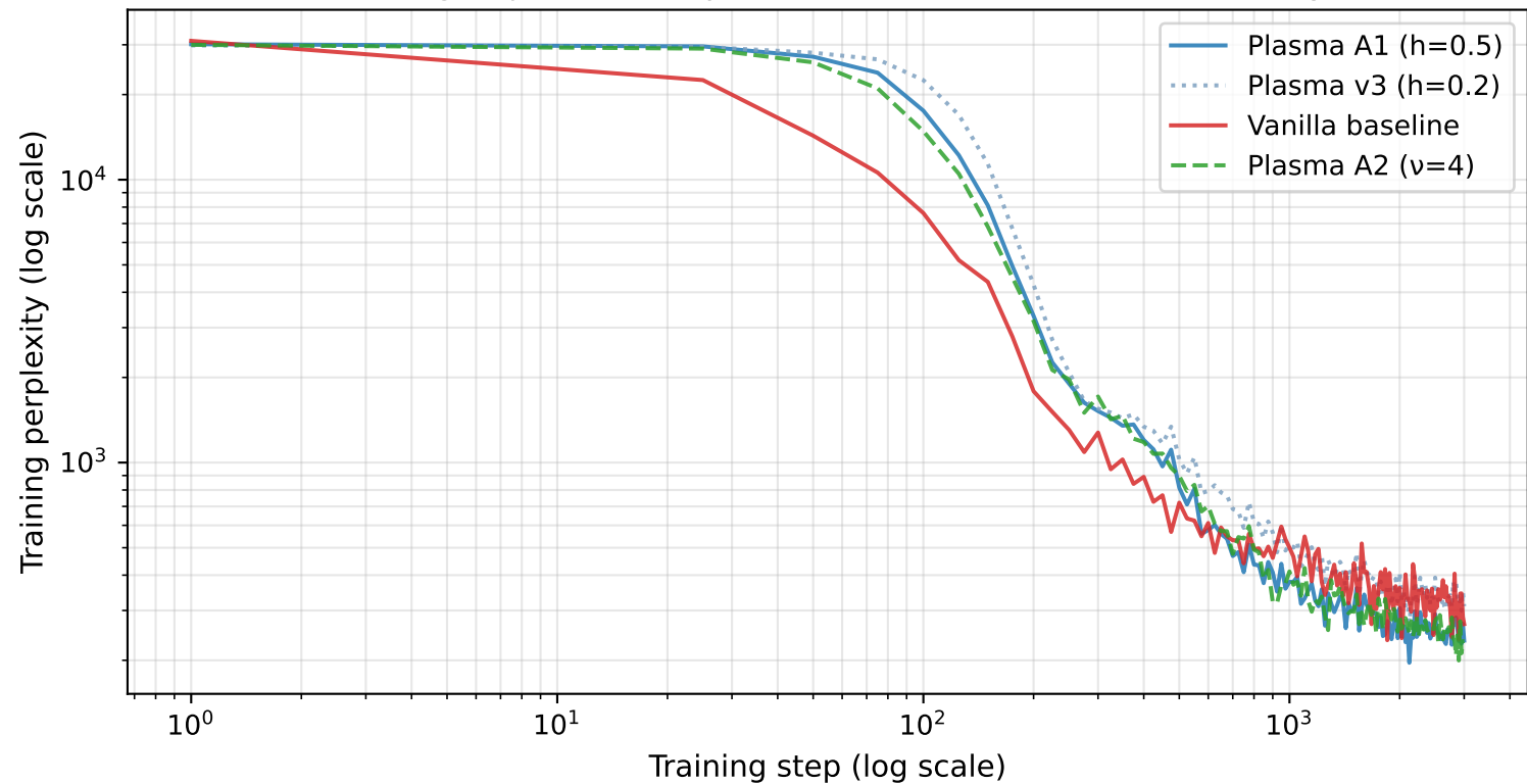
Training trajectories — plasma at h=0.5 tracks vanilla closely
