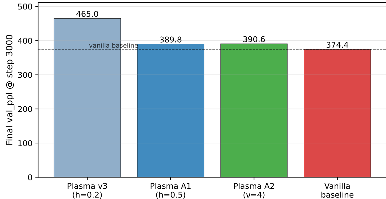
Ablation summary — h-step is the dominant recoverable factor
