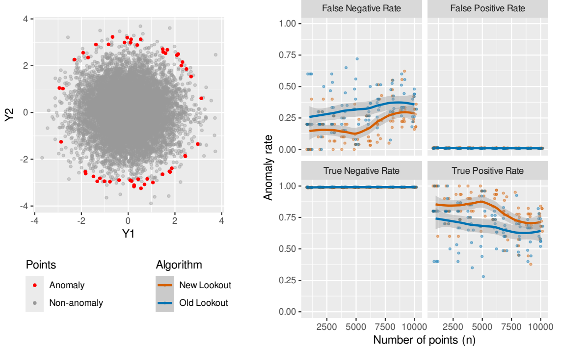
Fig. 3: Experiment 3 data and results using Normal distributions. Left: data for n = 10000 . Right: the relative performance of the two algorithms. The points in the right panel are slightly jittered horizontally to avoid overlapping points.
