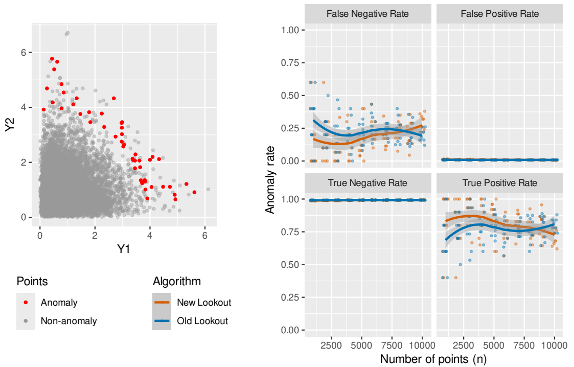
Fig. 4: Experiment 4 data and results using Gamma distributions. Left: data for n = 10000 . Right: the relative performance of the two algorithms. The points in the right panel are slightly jittered horizontally to avoid overlapping points.
