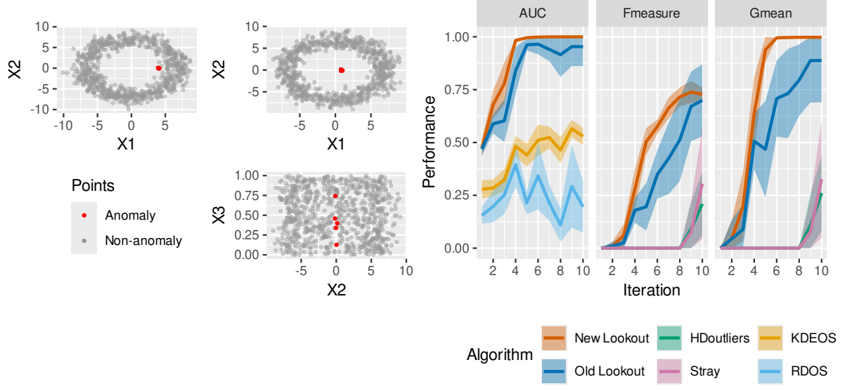
Fig. 9: Experiment 6 results. Top left: Data from the 3rd iteration showing the X_1X_2 plane with anomalies in red. Middle left: Data from the 9th iteration showing both the X_1X_2 plane and X_2X_3 plane, with anomalies moving into the annulus. Right: AUC, Fmeasure and Gmean of old and new versions of lookout, HDoutliers, KDEOS, RDOS and stray.
