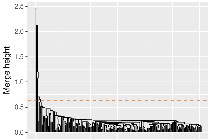
Single linkage dendrogram
