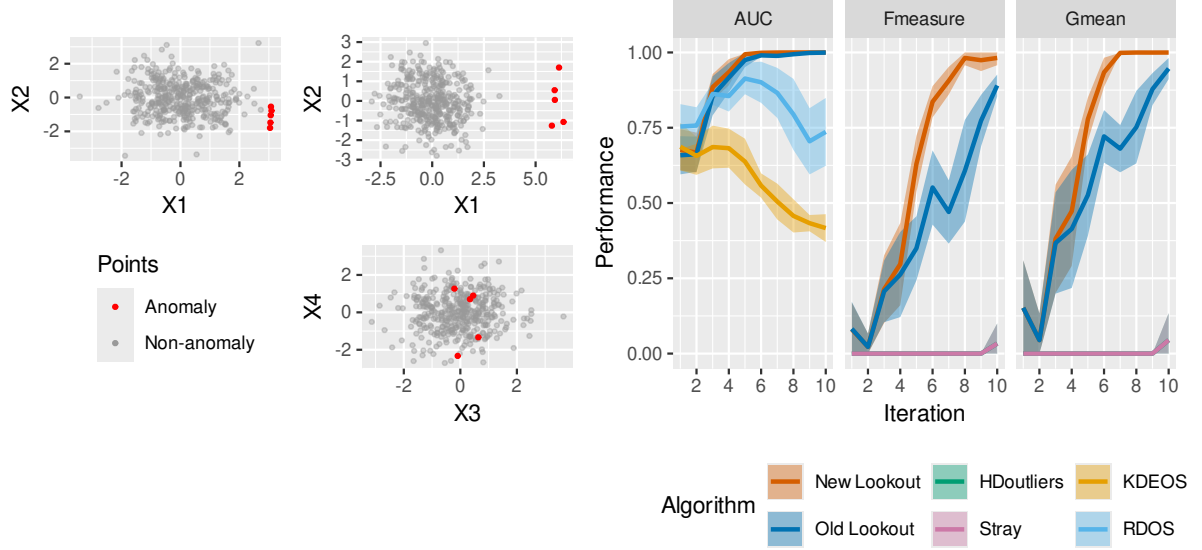
Fig. 8: Experiment 5 results. Top left: Data from the 3rd iteration showing the X_1 X_2 plane with anomalies in red. Middle left: Data from the 9th iteration showing both the X_1 X_2 plane and X_3 X_4 plane, with anomalies moving further away in the X_1 direction, resulting in the anomalies and non-anomalies being mixed on the X_3 X_4 plane. Right: AUC, Fmeasure and Gmean of old and new versions of lookout, HDoutliers, KDEOS, RDOS and stray.
