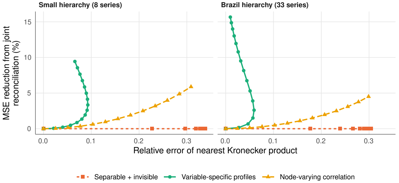
Figure 3: Experiment 1: population MSE reduction from joint rather than separate reconciliation against the relative error of the nearest Kronecker approximation to W .
