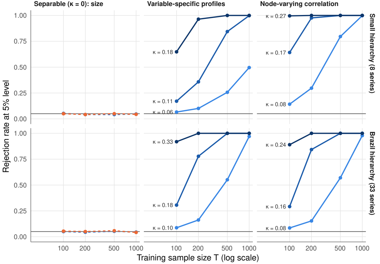
Figure 6: Experiment 1: rejection rate at the 5% level of the test of condition (d), by sample size (1000 replications). For the separable (F0) and separable-plus-invisible (F1) covariances the rejection rate is the size of the test.
