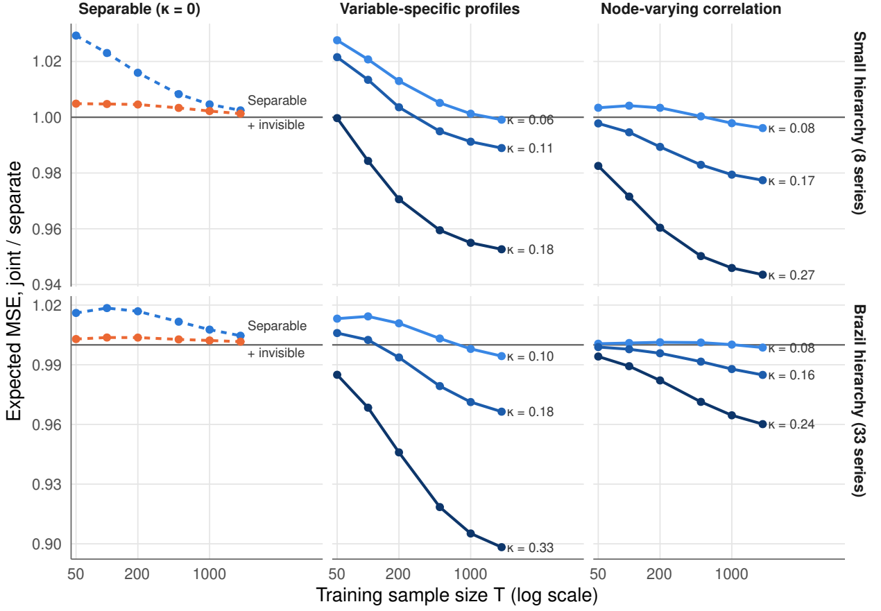
Figure 4: Experiment 1: expected MSE of joint relative to separate reconciliation with shrinkage estimates of W , by training sample size. Values below one favour joint reconciliation. Labels give the population \kappa .
