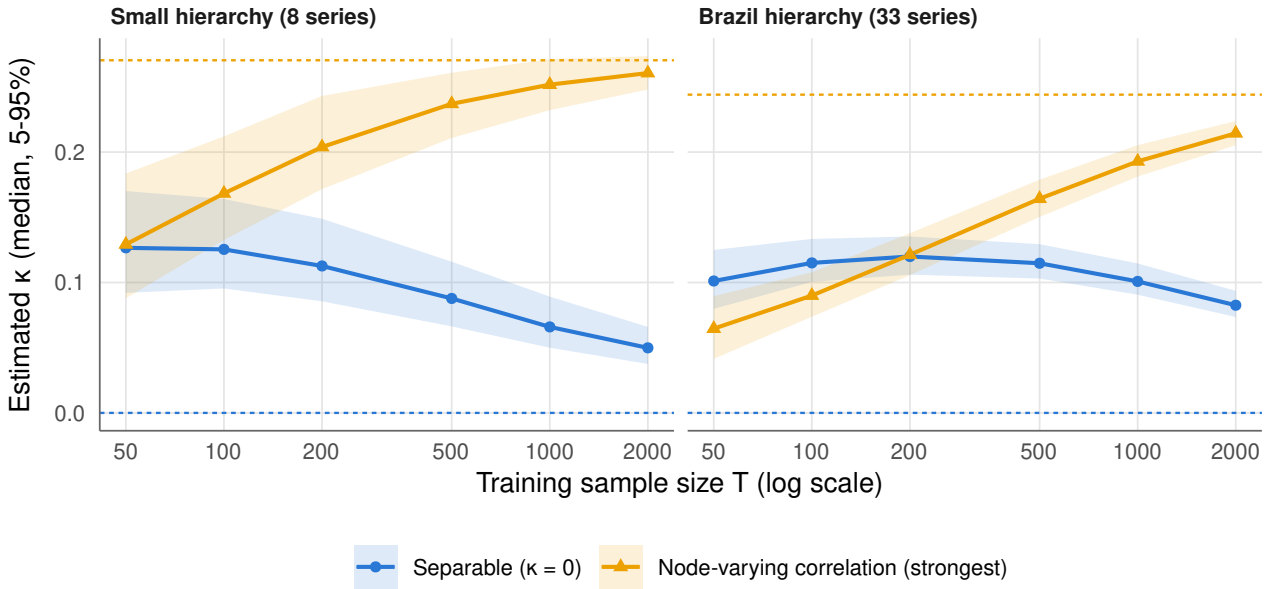
Figure 5: Experiment 1: sampling distribution of \hat{\kappa} (median and 5–95% range) under the separable family F0 and under the node-varying family F3 with the largest departure, with the population values dashed.
