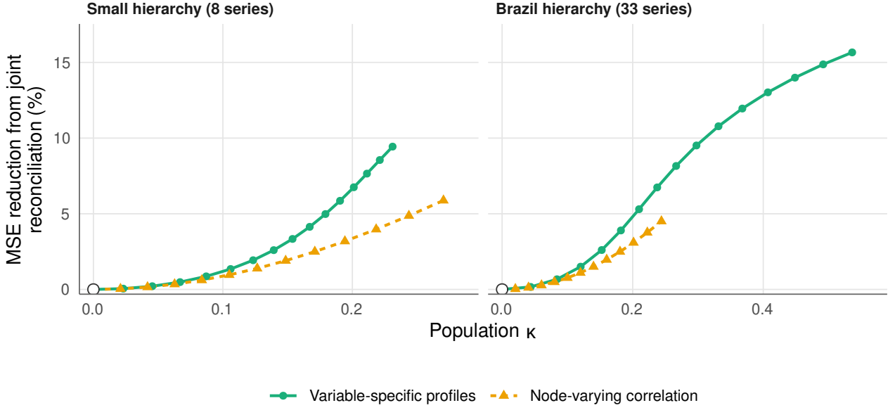
Figure 2: Experiment 1: population MSE reduction from joint rather than separate reconciliation against \kappa . The separable (F0), separable-plus-invisible (F1) and OLS (F4) families all lie at the origin.
