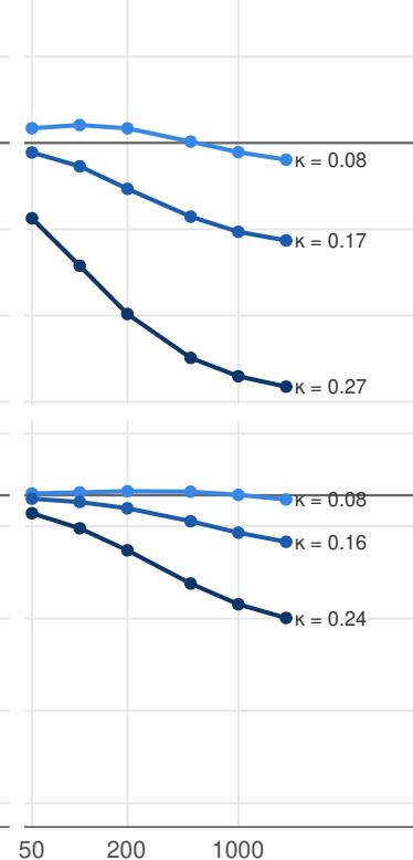
Node-varying correlation
