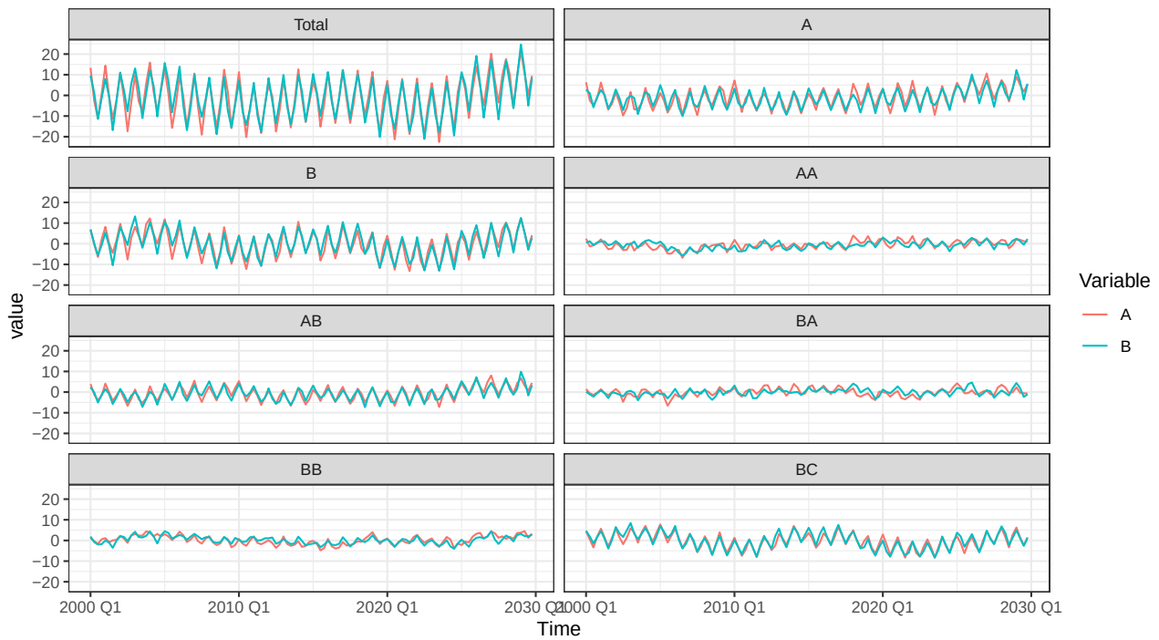
Figure S8: Simulation of a hierarchical multivariate time series, with the same structure as Figure 1, with m = 2 , under Scenario 8.
