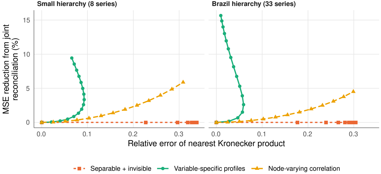
Figure 3: Experiment 1: population MSE reduction from joint rather than separate reconciliation against the relative error of the nearest Kronecker approximation to \mathbf{W} .
