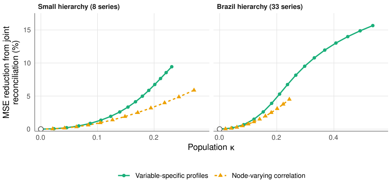
Figure 2: Experiment 1: population MSE reduction from joint rather than separate reconciliation against \kappa . The separable (F0), separable-plus-invisible (F1) and OLS (F4) families all lie at the origin.
