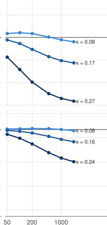
Node-varying correlation
