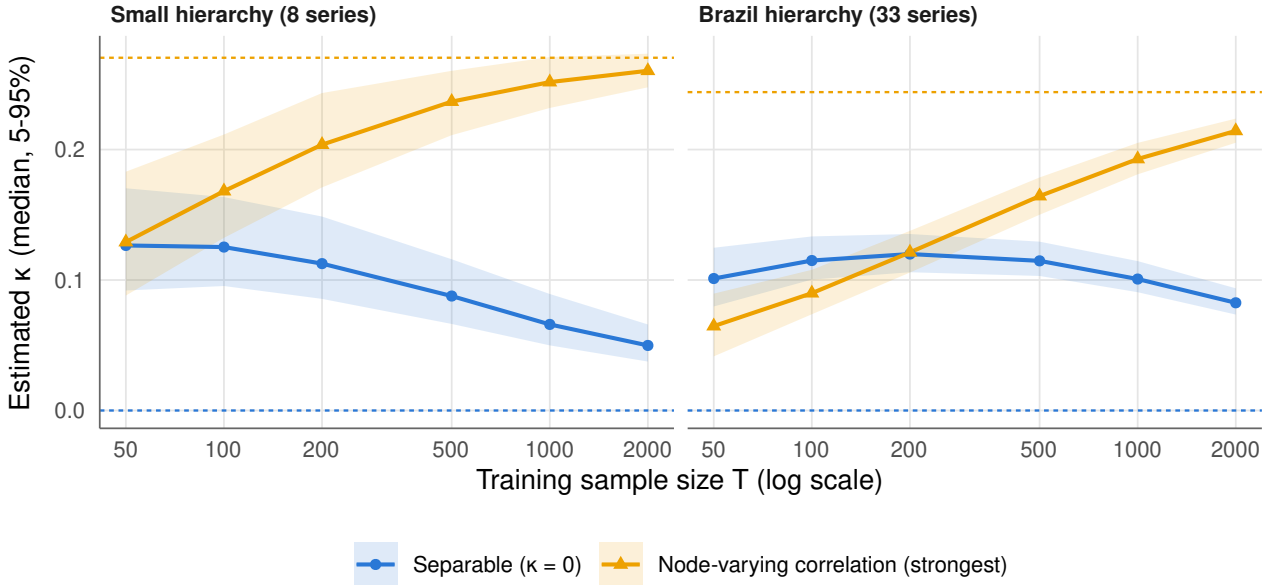
Figure 3: Sampling distribution of \widehat{\kappa} (median and 5–95% range over 1000 replications) under a separable covariance and under the strongest node-varying correlation case, with the population values dashed.
