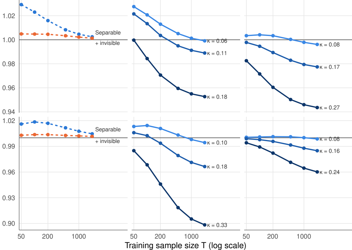
Separable ( \kappa = 0 )
