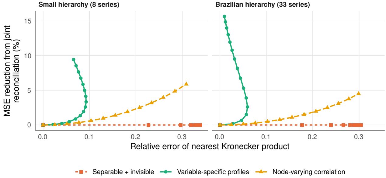
Figure 3: Experiment 1: population MSE reduction from joint rather than separate reconciliation against the relative error of the nearest Kronecker approximation to W . Each line joins the points for one family in order of its parameter, starting from the origin, where W is separable. For F1 the Kronecker error grows with the size of the invisible component while the gain stays at zero. For F2 the gain rises throughout, but the Kronecker error rises and then falls as \delta increases, so the line doubles back.
