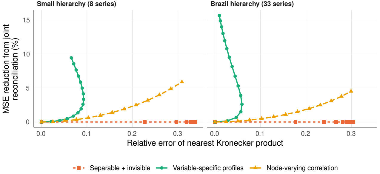
Figure 2: Population MSE reduction from joint reconciliation against the relative error of the nearest Kronecker approximation to W , for the covariance families of Section 5.
