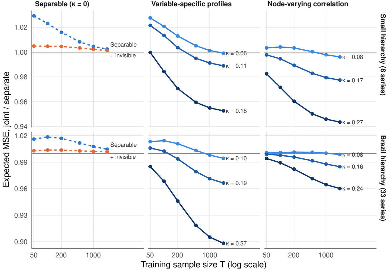
Figure 6: Experiment 1: expected MSE of joint relative to separate reconciliation with shrinkage estimates of W , by training sample size. Values below one favour joint reconciliation. Labels give the population \kappa .
