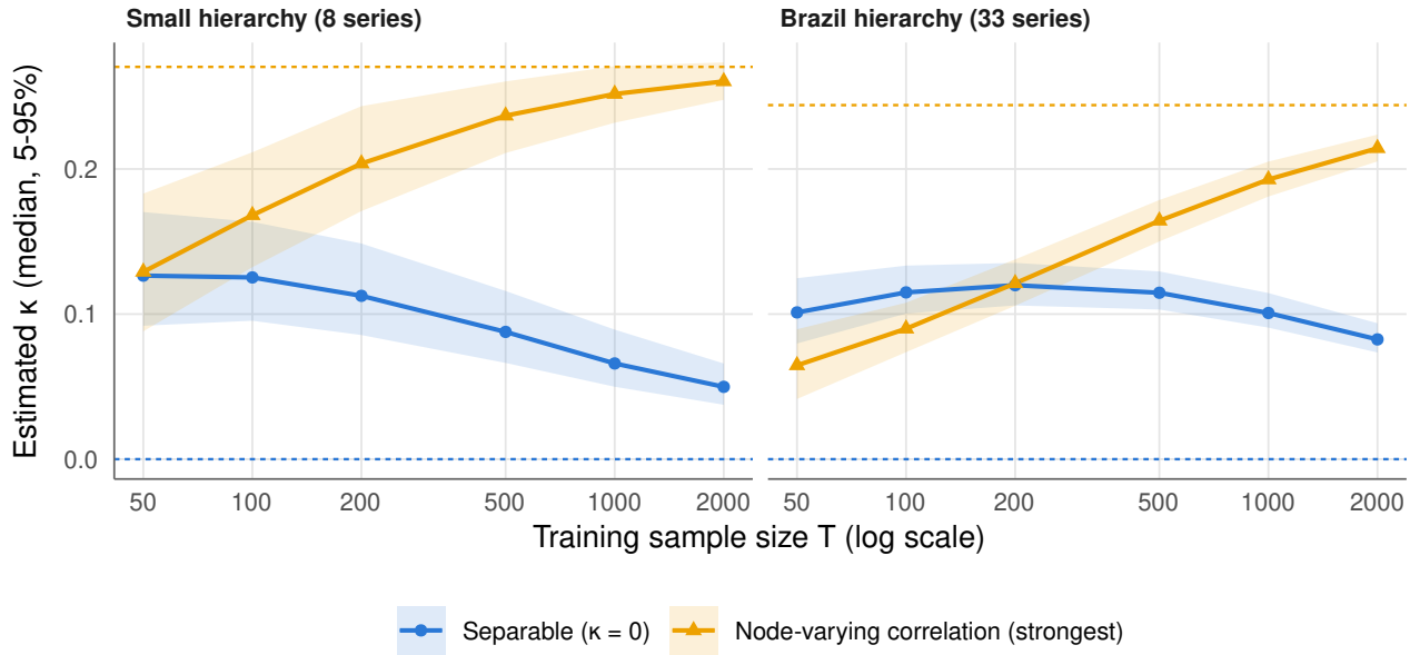
Figure 5: Experiment 1: sampling distribution of \hat{\kappa} (median and 5–95% range) under the separable family F0 and under the node-varying family F3 with the largest departure, with the population values dashed.
