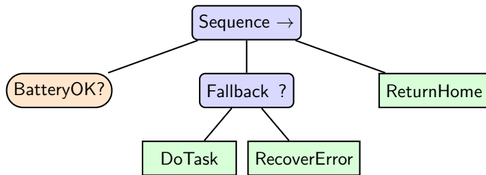
Figure 6: A small behavior tree, with a Sequence root, a nested Fallback subtree, an action ( \square ), a condition ( \circ ) and a recovery alternative.
