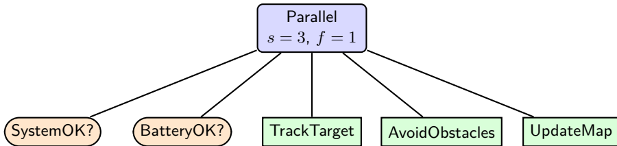
Figure 8: A Parallel node with thresholds \text{min\_success}=3 and \text{min\_failure}=1 : the subtree succeeds as soon as any three children succeed (supposedly, the first three), and fails as soon as any child fails; every remaining RUNNING child is halted.
