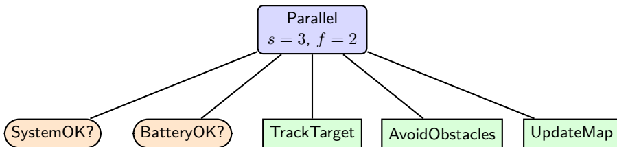
Figure 8: A Parallel node with thresholds \text{min\_success}=3 and \text{min\_failure}=2 : the subtree succeeds as soon as any three children succeed, and fails as soon as any two children fail; every remaining RUNNING child is halted.
