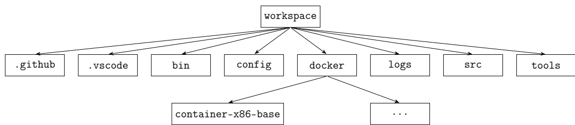
Figure 4.2: Directory tree of a DUA unit based on dua-template [127].
