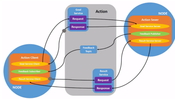
Figure 3.8: Scheme of the action communication primitive [190].
