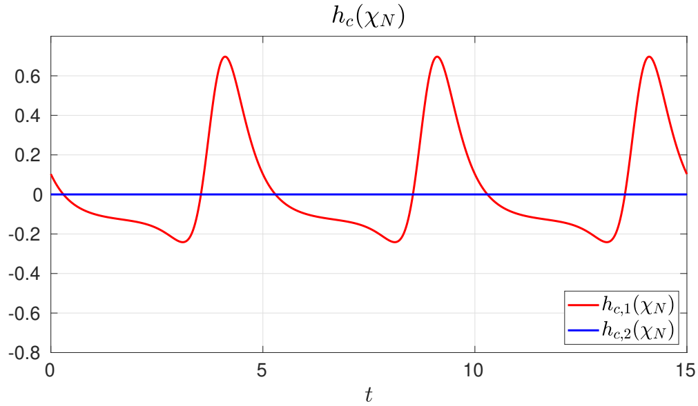
Figure 7.9: Nominal feedback-linearizing system input.
