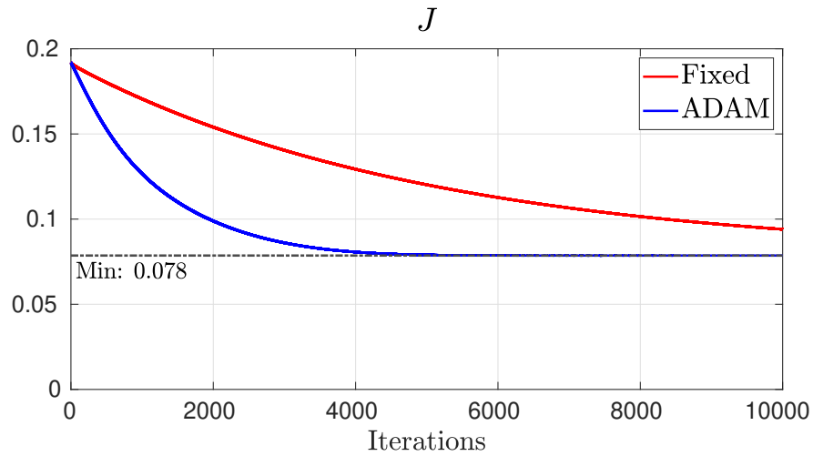
Figure 7.8: Cost during all the iterations performed with Algorithm 1 (red) versus those with Algorithm 2 (blue).
