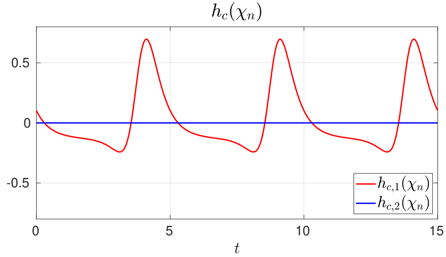
Figure 7.9: Nominal feedback-linearizing system input.
