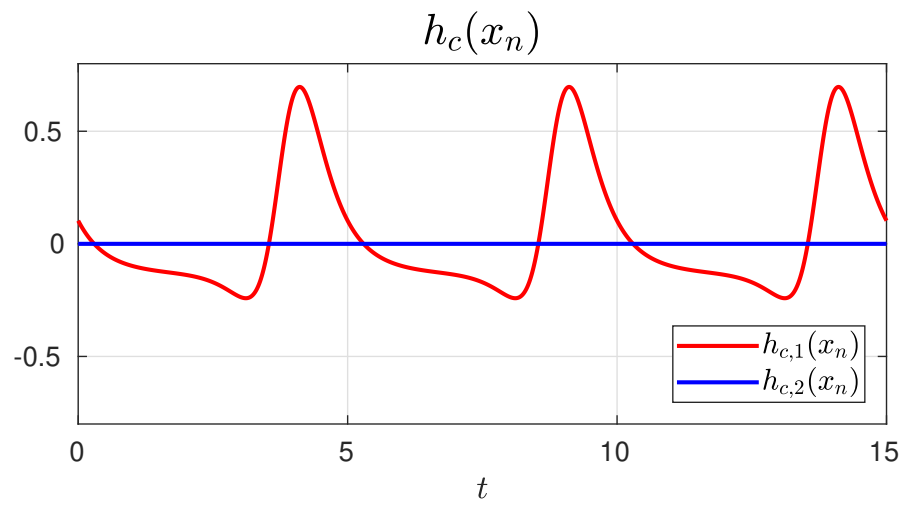
Figure 7.9: Nominal, feedback-linearizing control law.
