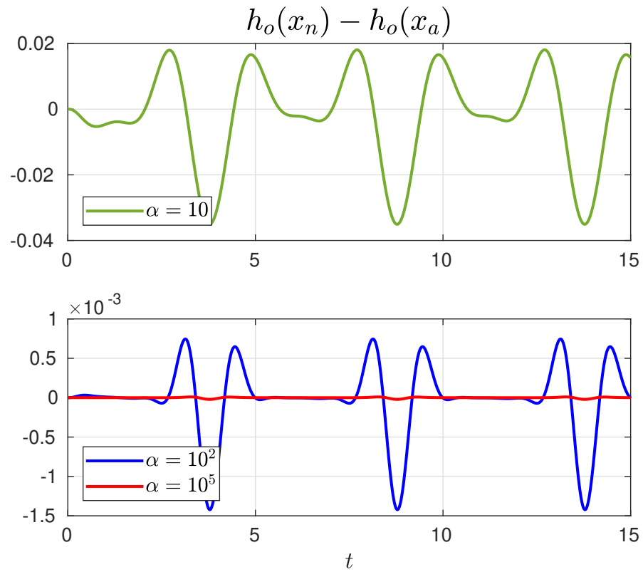
Figure 7.7: Difference between the system output with and without input allocation, for different values of the invisibility weight \alpha , during the final run of Algorithm 1.
