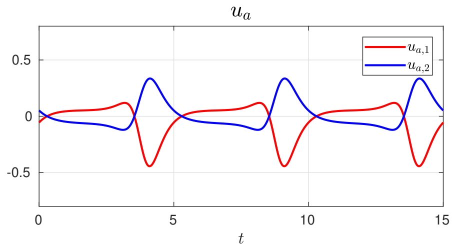
Figure 7.10: Optimal auxiliary input determined by Algorithm 2.
