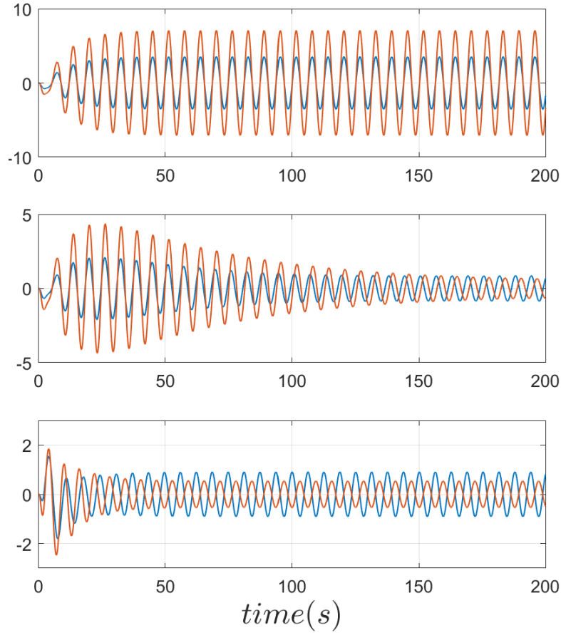
Figure 7.13: ( Nominal case ) Top graph: time histories of y_c(t) , i.e. , the non-allocated control input. Middle and bottom graphs: time histories of u(t) = y_c(t) + \varsigma(t) , i.e. , the optimally-allocated control input, with \gamma = 0.01 and \gamma = 0.1 . The steady-state values in the middle and bottom graphs are the same, but a larger \gamma yields a faster convergence.
