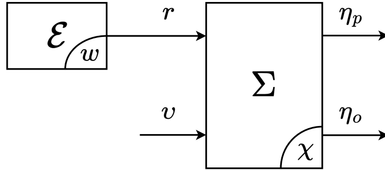
Figure 7.1: Block diagram of the system \Sigma in eq. (7.1) interconnected to the exosystem \mathcal{E} in eq.(7.2).
