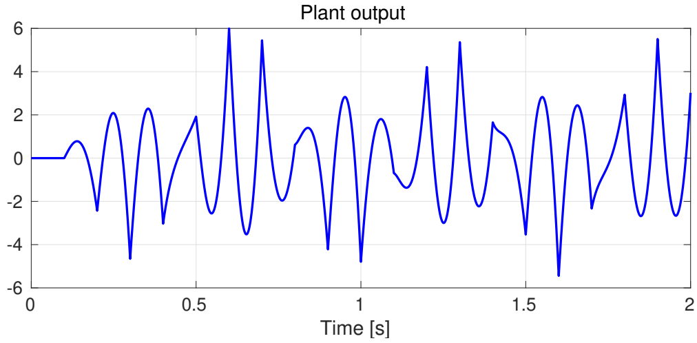
Figure 7.20: Output of the continuous-time, linear time-invariant plant (7.153) in presence of its polynomial annihilator subject to the sinusoidal input (7.154).
