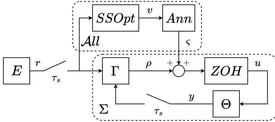
Figure 7.18: Sampled-data feedback control system given by (7.142)–(7.145) interconnected as in (7.149), and (7.147)–(7.148); the discrete-time allocator is enclosed in the \mathcal{A}ll block.
