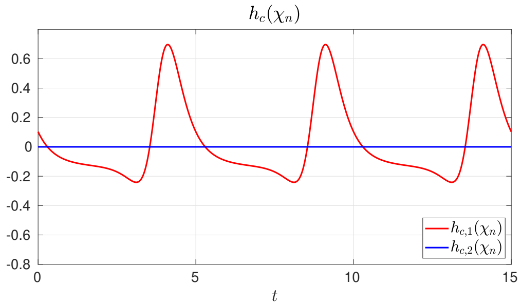
Figure 7.9: Nominal feedback-linearizing system input.
