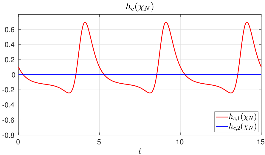
Figure 7.9: Nominal feedback-linearizing system input.
