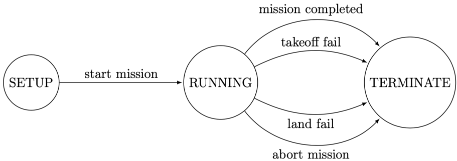
Figure 5.4: High-level finite-state machine for the Leonardo Drone Contest 2021 mission.
