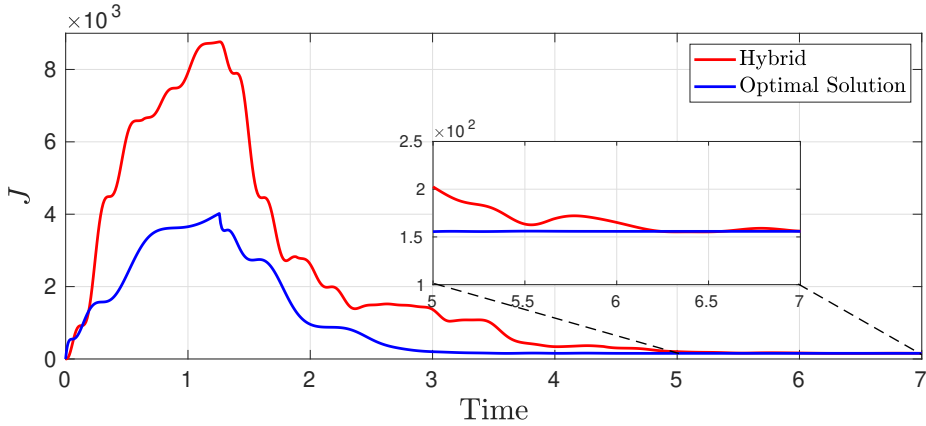
Figure 7.4: Cost in the presence of input allocation by means of a hybrid allocator (red), and of the periodic extension of the optimal solution to Problem 7.11 (blue). The last value is the relevant one.
