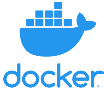
Figure 3.14: Docker logo [60].
