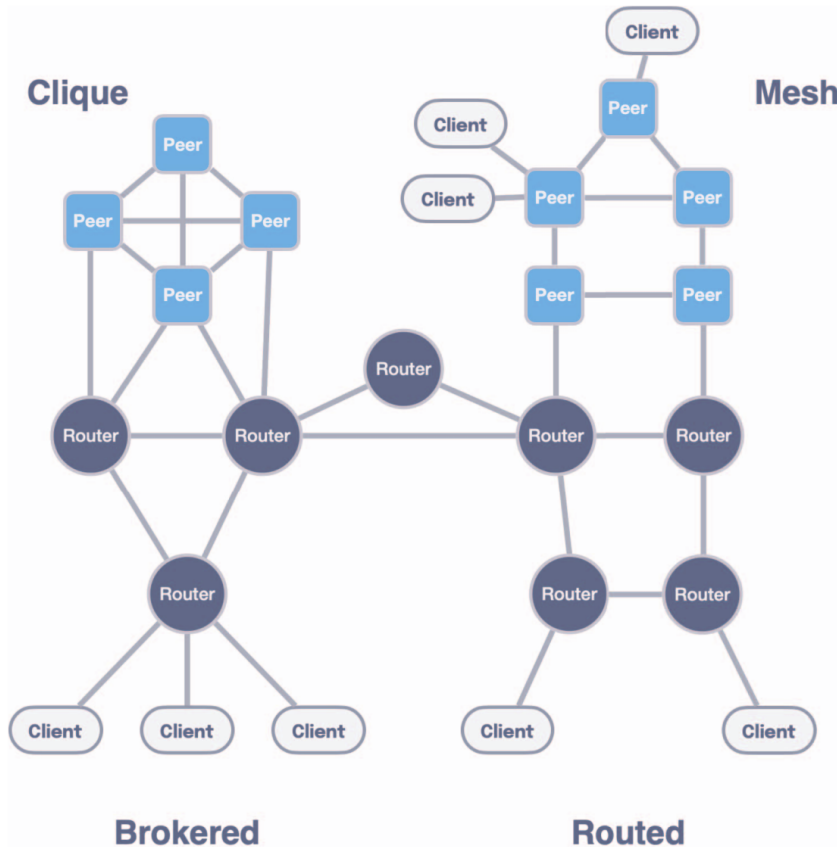
Figure 3.3: Possible network topologies in Zenoh [50].
