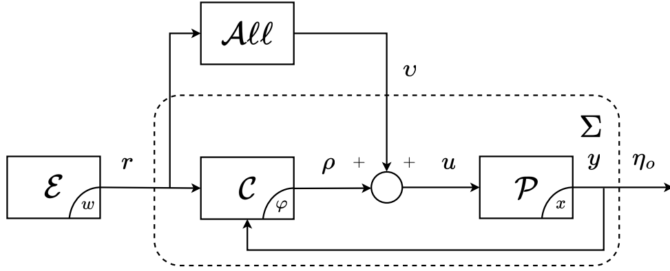
Figure 7.3: Block diagram of the feedback control system \Sigma given by eq. (7.7), (7.8), and (7.9); the input allocation device is enclosed in the \mathcal{A}ll block.
