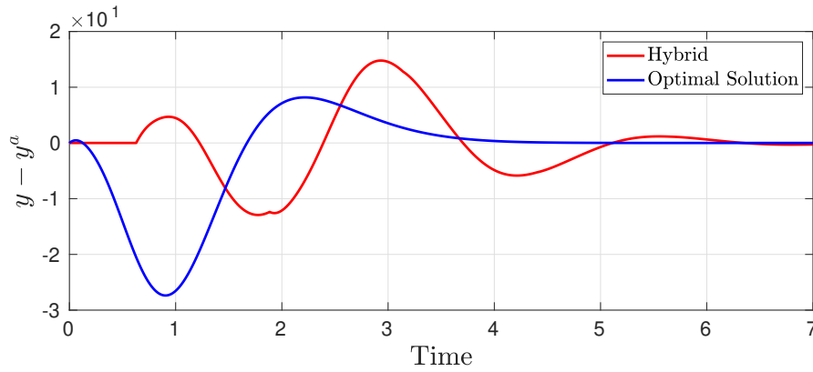
Figure 7.5: Differences between the outputs of the non-allocated and allocated closed loops, in the presence of a hybrid allocator (red) and of the periodic extension of the optimal solution to Problem 7.3 (blue).
