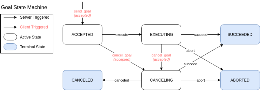
Figure 3.9: State machine of an action goal [23].
