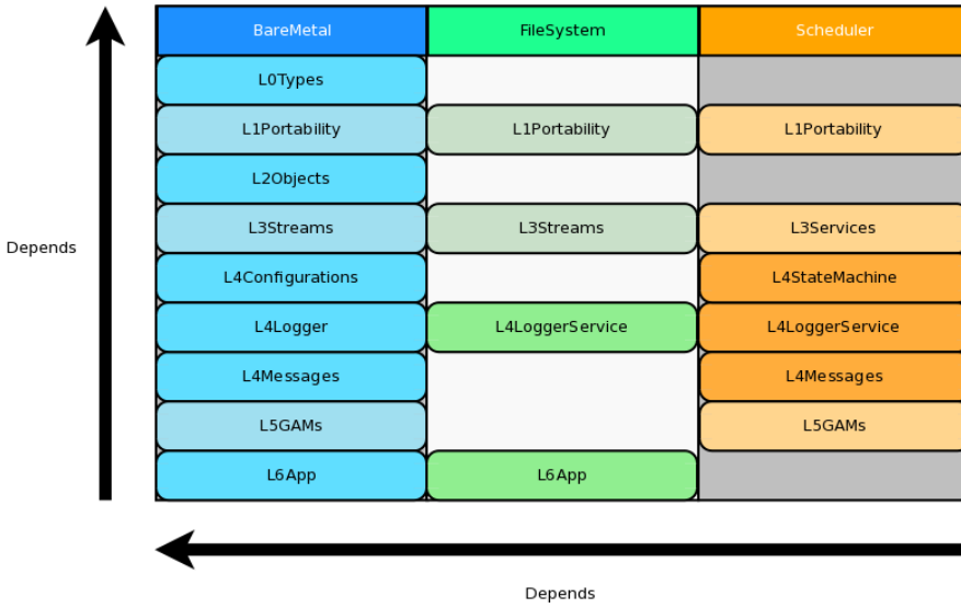
Figure 2.1: Organization of the core libraries of the MARTe2 framework [83].
