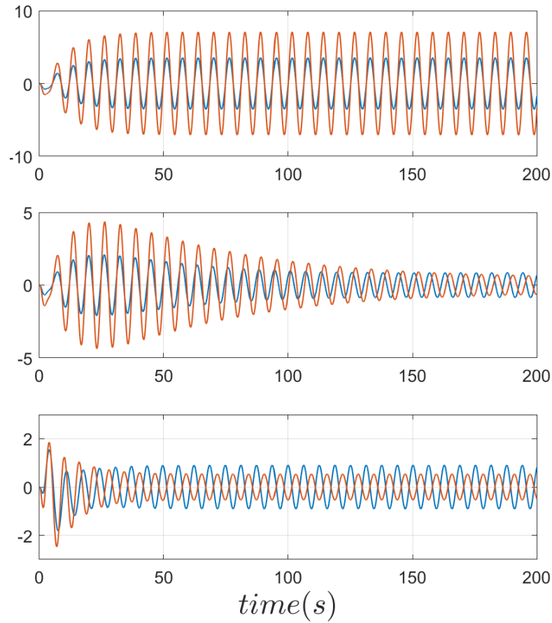
Figure 7.13: ( Nominal case ) Top graph: time histories of y_c(t) , i.e. , the non-allocated control input. Middle and bottom graphs: time histories of u(t) = y_c(t) + \zeta(t) , i.e. , the optimally-allocated control input, with \gamma = 0.01 and \gamma = 0.1 . The steady-state values in the middle and bottom graphs are the same, but a larger \gamma yields a faster convergence.
