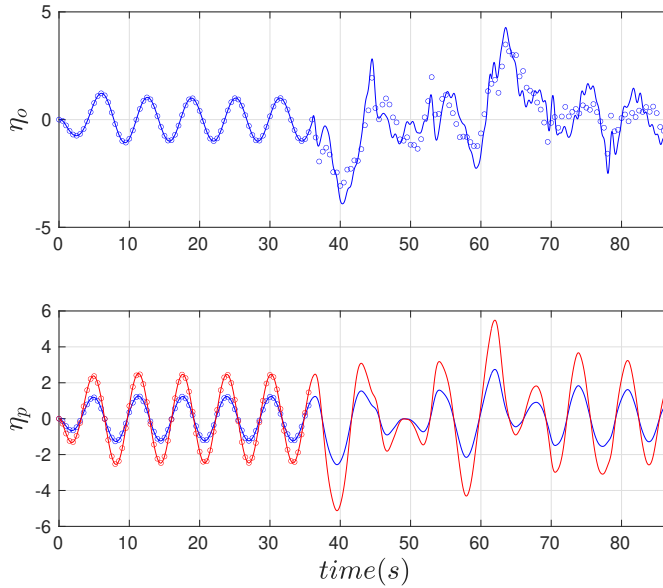
Figure 7.14: ( Uncertain case ) Regulated (top graph) and performance (bottom graph) outputs of the uncertain plant during the two-phase identification process. The markers on each plot identify the sampling times and the values used by the data-driven procedures. In the last part of the upper plot, the markers show the values of \eta_o^\delta(k\tau_s) (see line 8 of Algorithm 6).
