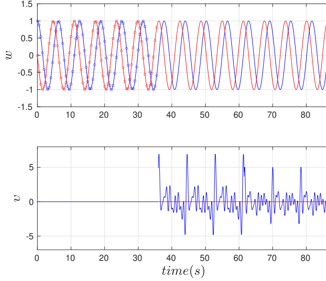
Figure 7.15: ( Uncertain case ) Time histories of the reference input (top graph) and of the controlled input (bottom graph) during the two-phase identification process. The markers identify the sampling times.
