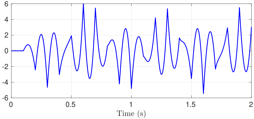
Figure 7.20: Output of the continuous-time, linear time-invariant plant (7.153) in presence of its polynomial annihilator subject to the sinusoidal input (7.154).
