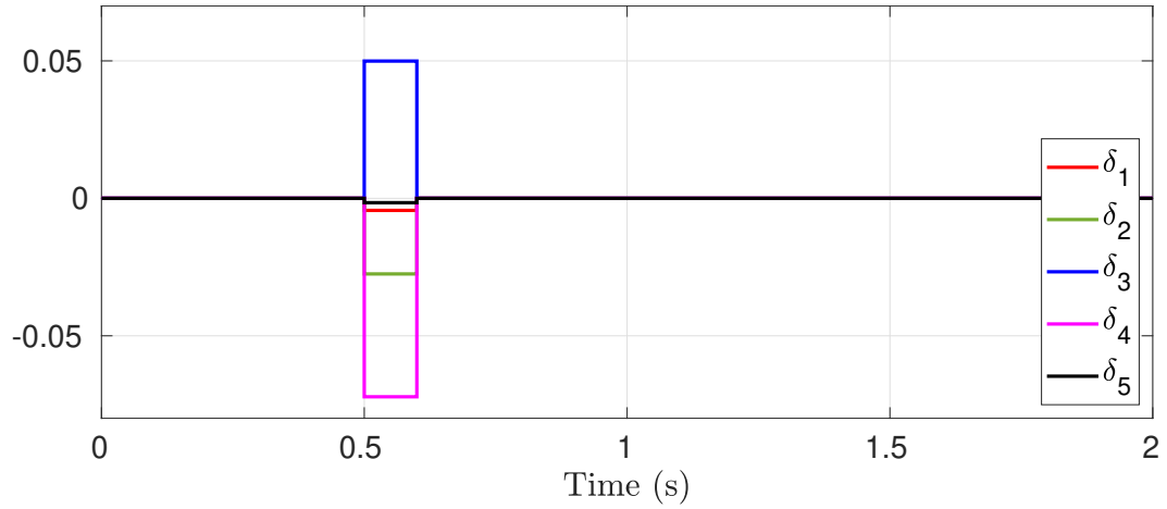
Figure 7.22: Steady-state optimizer correction term \delta .
