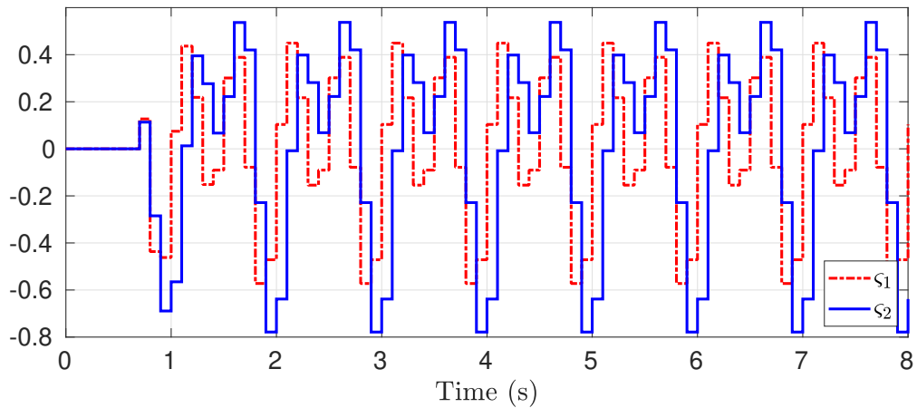
Figure 7.24: Discrete-time allocator output \varsigma .
