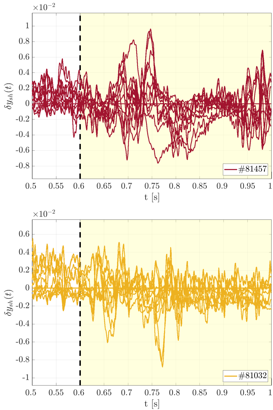
Figure 7.31: Time histories of the components of the shape error e_{sh} for pulses #81457 with the dynamic annihilator (top) and #81032 with the static annihilator (bottom).
