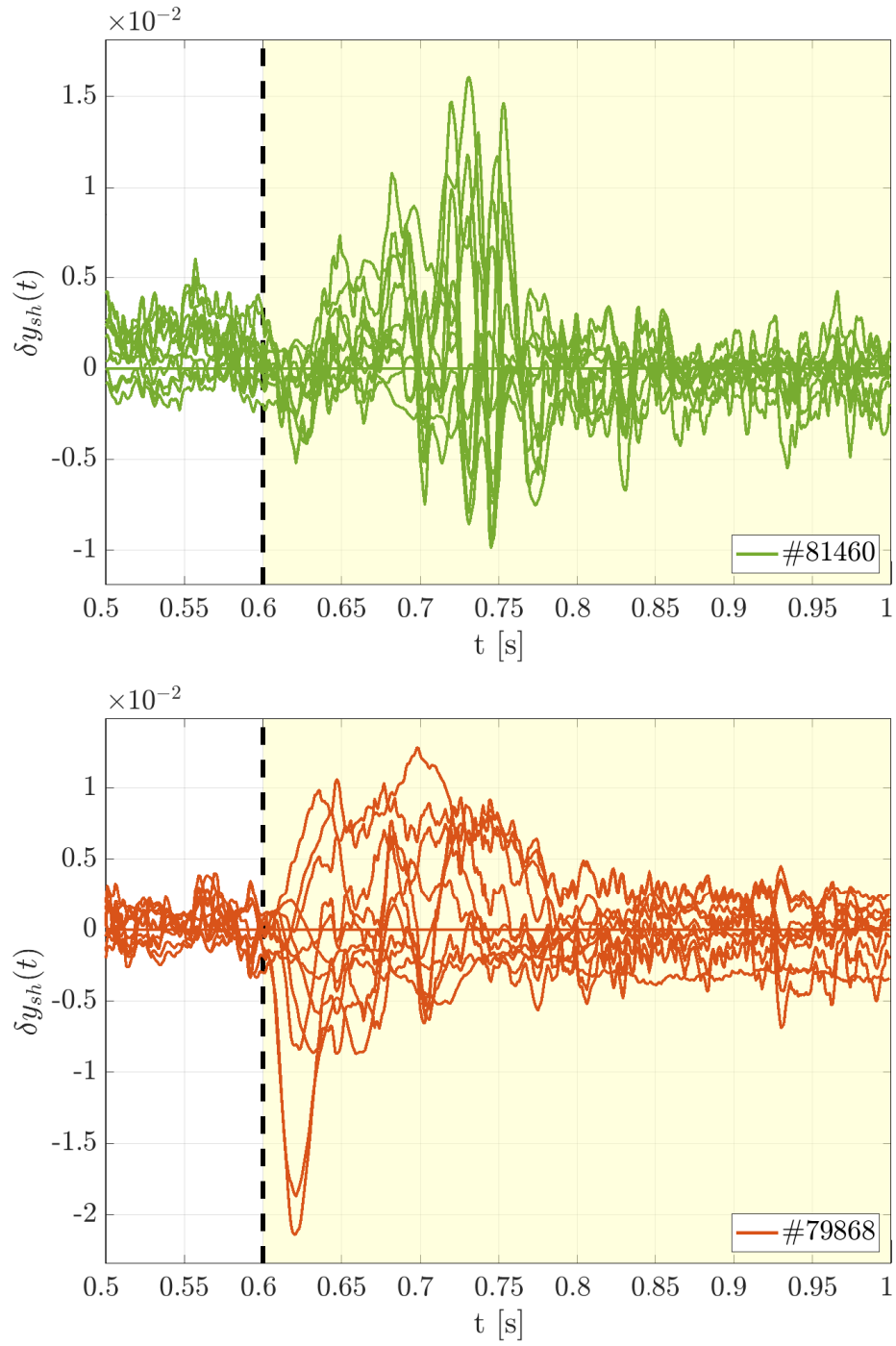
Figure 7.35: Time histories of the components of the shape error e_{sh} for pulses #81460 with the dynamic annihilator (top) and #79868 with the static annihilator (bottom).
