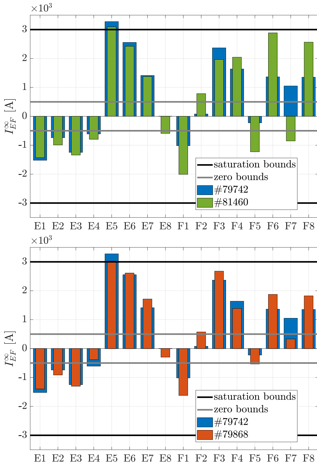
Figure 7.33: Steady-state values of the EF coil currents for pulses #81460 (top) and #79868 (bottom) against the reference pulse #79742.
