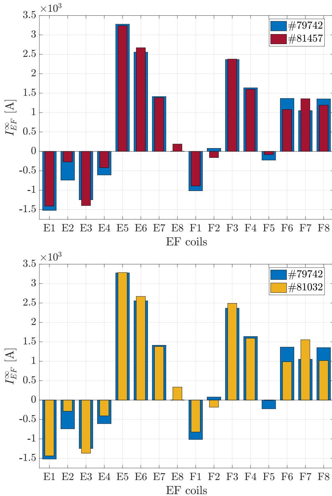
Figure 7.29: Steady-state values of the EF coil currents for pulses #81457 (top) and #81032 (bottom) against the reference pulse #79742.
