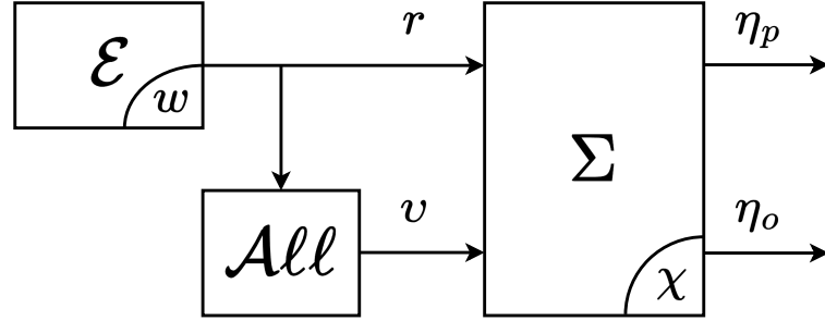
Figure 7.2: Block diagram of the system \Sigma given by eq. (7.1) interconnected to the exosystem \mathcal{E} defined in eq. (7.2) and to the input allocation device, enclosed in the All block.
