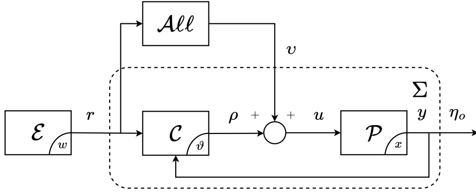
Figure 7.3: Block diagram of the feedback control system \Sigma given by eq. (7.7), (7.8), and (7.9); the input allocation device is enclosed in the All block.
