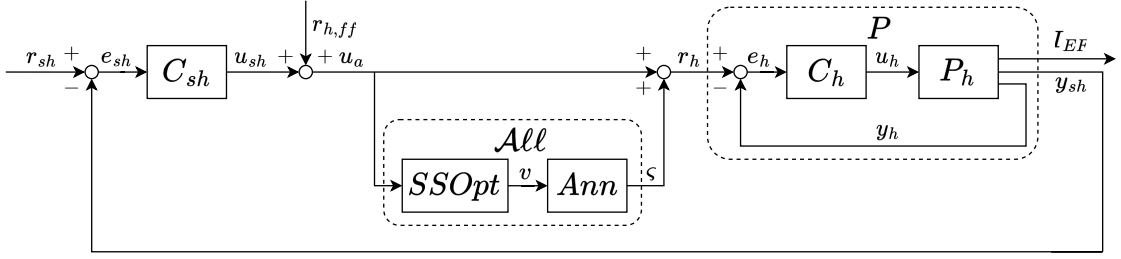
Figure 7.27: Simplified diagram of the TCV control scheme: the P_h block represents the actual plant, couple with the hybrid feedback controller C_h ; the shape controller is represented by the C_{sh} block, whereas the proposed allocator is embedded in the \mathcal{A}ll block.
