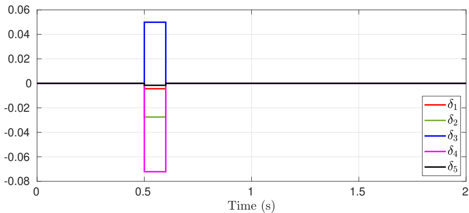
Figure 7.22: Steady-state optimizer correction term \delta .
