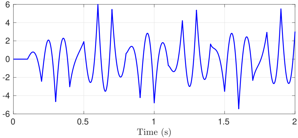
Figure 7.20: Output of the continuous-time, linear time-invariant plant (7.155) in presence of its polynomial annihilator subject to the sinusoidal input (7.156).
