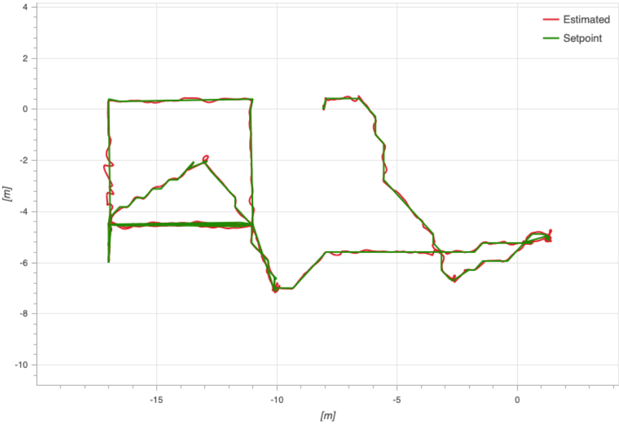
Figure 5.8: 2021 Leonardo Drone Contest mission run; the green path represents the setpoints while the red one represents the estimated trajectory.
