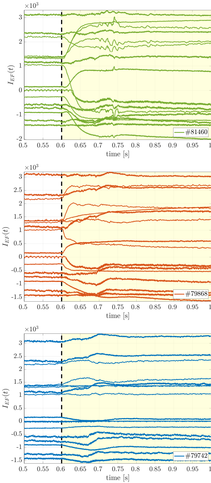
Figure 7.34: Time histories of the EF coil currents for pulses #81460 (top), #79868 (middle), and #79742 (bottom).
