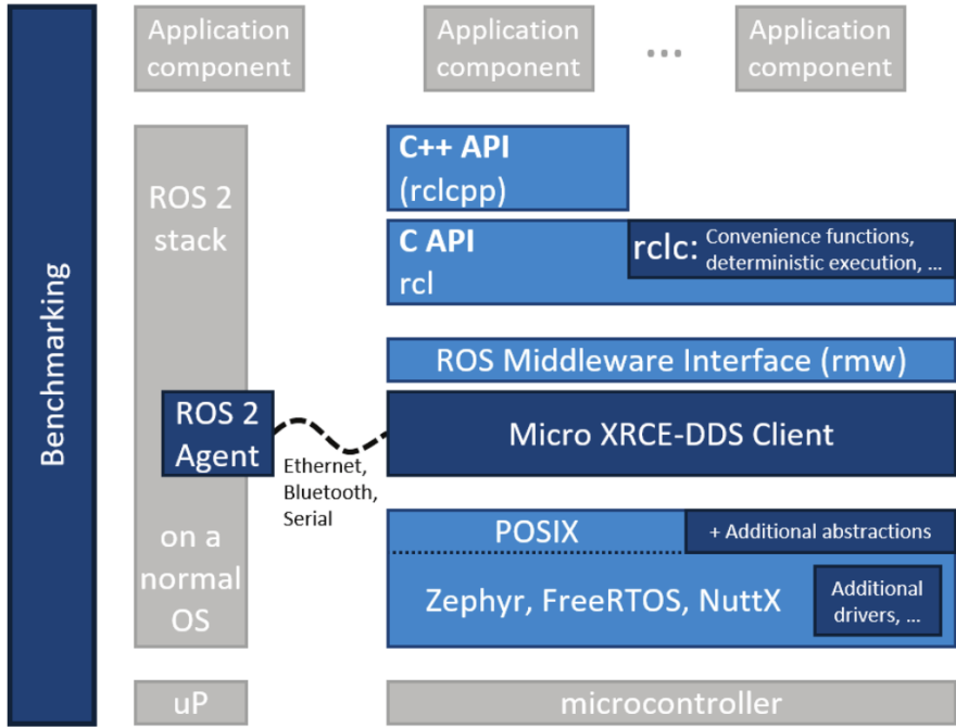
Figure 3.13: micro-ROS architecture [72].
