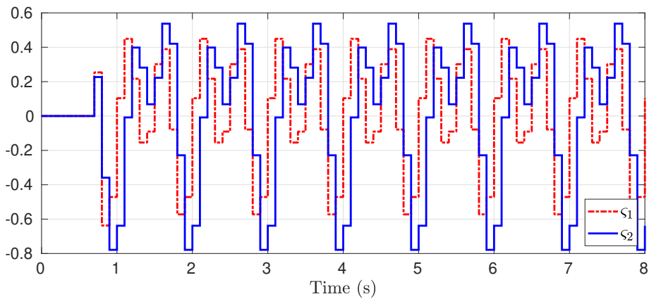
Figure 7.24: Discrete-time allocator output \varsigma .
