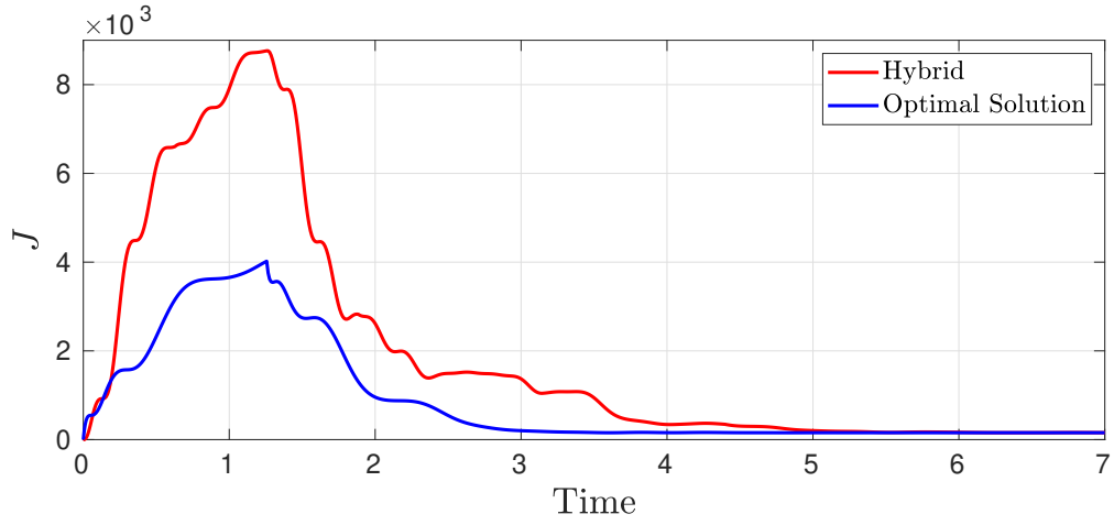
Figure 7.4: Cost in the presence of input allocation by means of a hybrid allocator (red), and of the periodic extension of the optimal solution to Problem 7.10 (blue).
