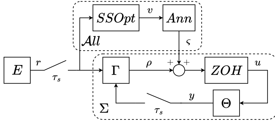
Figure 7.18: Sampled-data feedback control system given by (7.143)–(7.146) interconnected as in (7.150), and (7.148)–(7.149); the discrete-time allocator is enclosed in the \mathcal{A}ll block.
