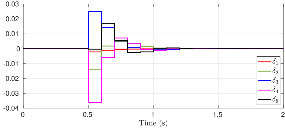
Figure 7.25: Optimizer correction term \delta smoothed by \alpha = 0.5 (see Remark 7.69).
