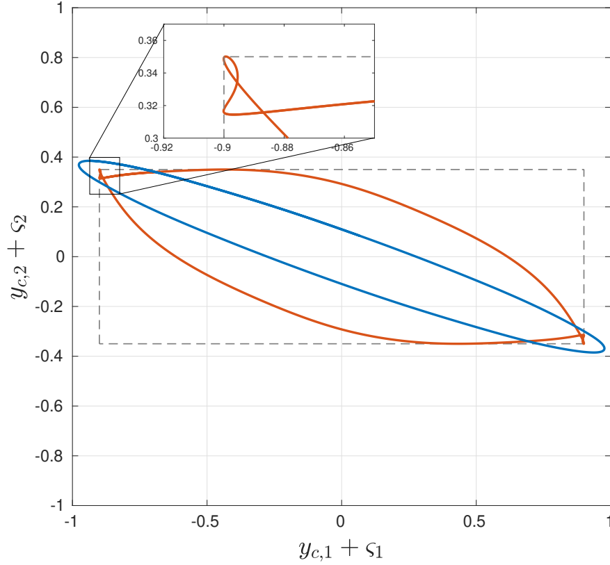
Figure 7.16: ( Deadzone ) Behavior of the allocated control inputs, together with the deadzone representation (dashed gray box). The control actions allocated via an allocator with \text{spec}(A_{IM}) = \bigcup_{\kappa=1}^4 \text{spec}(\kappa S) (red graph) achieve further amplitude reduction compared to an allocator with \text{spec}(A_{IM}) = \text{spec}(S) (blue graph) (see Figure 7.17).
