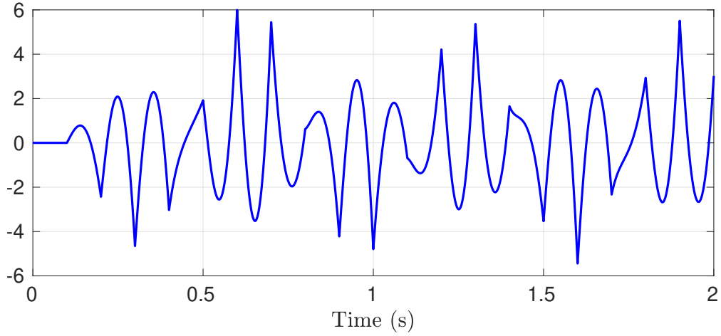
Figure 7.20: Output of the continuous-time, linear time-invariant plant (7.154) in presence of its polynomial annihilator subject to the sinusoidal input (7.155).
