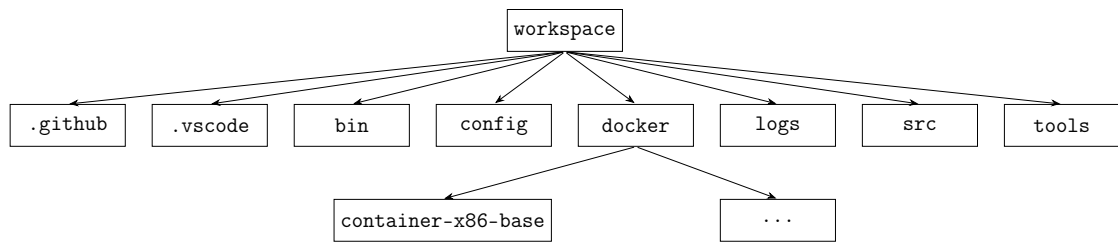
Figure 4.2: Directory tree of a DUA unit based on dua-template [14].
