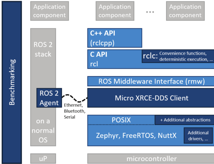
Figure 3.13: micro-ROS architecture [72].
