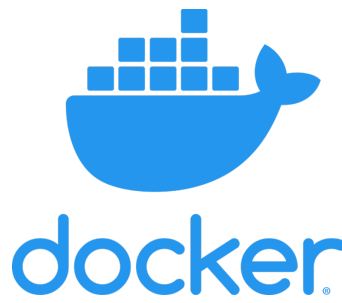
Figure 3.14: Docker logo [57].
